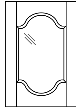
403GL-MDF Double Cathedral Minimum Width: 10 13/16" Minimum Height: 12"
