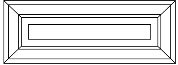
552 MR-2 DF Square Raised Minimum Width: 7 1/2" Minimum Height: 6 1/2"
