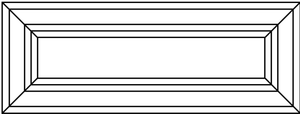
1053 MR-3 DF Square Reversed Raised Minimum Width: 7 1/2" Minimum Height: 6 1/2"
