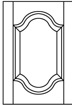
103 Double Cathedral Minimum Width: 9 3/4" Minimum Height: 12"
