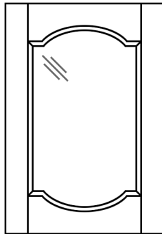
607GL Double Shoulder Eyebrow Minimum Width: 7 1/2" Minimum Height: 12"
