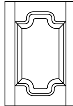
109 Double Flattop Minimum Width: 9 3/4" Minimum Height: 12"
