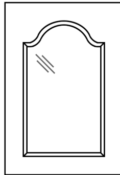
402GL-MDF Cathedral Minimum Width: 10 13/16" Minimum Height: 10"
