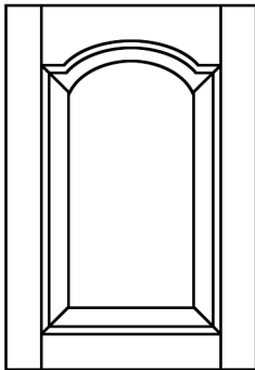
106 Shoulder Eyebrow Minimum Width: 9 3/4" Minimum Height: 10"
