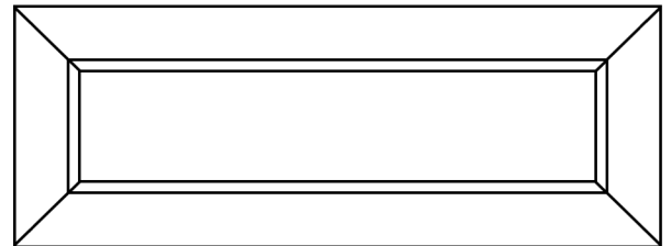
753 MR-3 DF Square Flat Minimum Width: 7 1/2" Minimum Height: 4 1/2"
