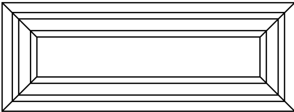
751 MR-1 DF Square Flat Minimum Width: 7 1/2" Minimum Height: 4 1/2"
