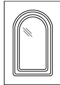
306GL-MDF Full Arch Minimum Width: 9" Minimum Height: 10"
